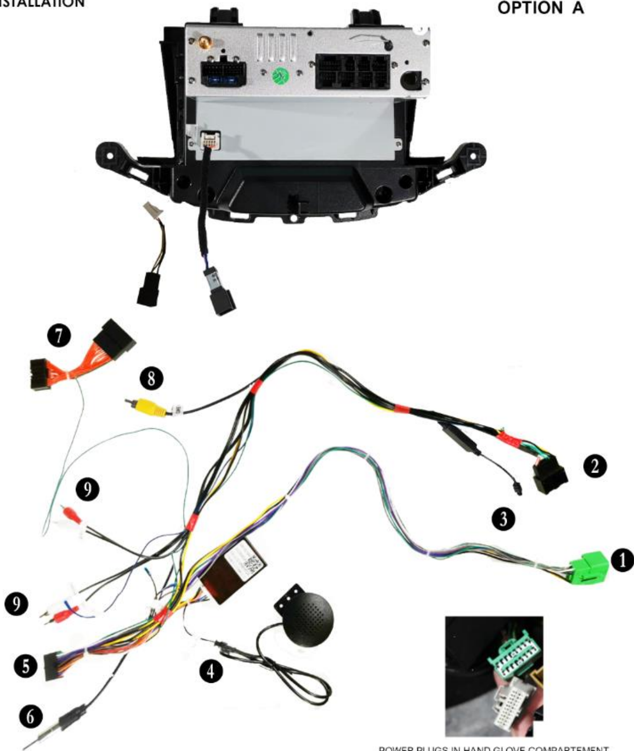
POWER PLUGS IN HAND GLOVE COMPARTMENT CONNECT TO PLUGS 6 & 7
